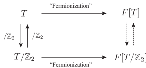
Figure 4: The interplay between fermionization and gauging \mathbb{Z}_2 symmetry. The downward arrow on the left denotes gauging the \mathbb{Z}_2 (n-1) -form symmetry in T , while the upward arrow on the left denotes gauging the dual \mathbb{Z}_2 (n-1) -form symmetry in F[T] . On the right, the downward arrow and upward arrow denotes stacking with the invertible phase in Section 4 or its complex conjugate, together with a change in the symmetry fractionalization as discussed in (96).
