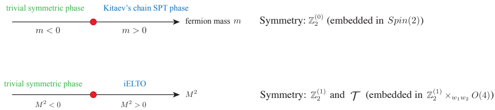
Figure 3: The upper diagram describes the phase transition of massless Majorana fermion in 1+1d with the fermion parity symmetry \mathbb{Z}_2^{(0)} embedded in the full space-time Spin(2) symmetry. This phase transition separates the trivial phase and the Kitaev's chain invertible fermionic phase. The free Majorana fermion in 1+1d is also dual to the \mathbb{Z}_2 gauge theory with the discrete theta angle (6), and the gauge field couples to a real scalar that has a quartic potential (for a review, see e.g. (2.9) of [55], where the \mathbb{Z}_2 gauge field is denoted by s , and the discrete theta angle is denoted by \frac{\pi}{2} \int q_\rho(s) = \pi \int \text{Arf}(s \cdot \rho) + \text{Arf}(\rho) with spin structure \rho ), which is the 1+1d analogue of the action (82). The mass square of the real scalar is identified with the fermion mass m with appropriate sign. The lower diagram describes the phase transition with exotic loops, which has \mathbb{Z}_2^{(1)} one-form symmetry and the (modified) time-reversal symmetry \mathcal{T} that are both embedded in the spacetime two-group symmetry \mathbb{Z}_2^{(1)} \times_{w_1 w_2} O(4) . The two sides of the phase transition are given by the trivial phase and the iELTO phase respectively. A proposed theory of this transition is given in (82). In both phase diagrams, the symmetry is unbroken on both sides of the phase transition, and thus the symmetry is also unbroken at the phase transition.
