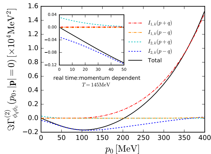
Figure 9: Imaginary part of the two-point correlation function \Gamma_{\phi_q \phi_c}^{(2)}(p_0, |\mathbf{p}| = 0) in the IR limit k \rightarrow 0 as a function of p_0 at temperature T = 145 MeV. Different contributions and the total one are shown, respectively. The inlay shows the zoomed-in view in the region of small p_0 .
