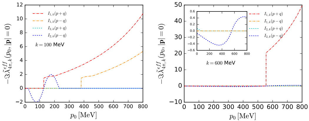
Figure 8: Different parts of contribution to the imaginary part of -\tilde{\lambda}_{4\pi,k}^{\text{eff}}(p_0, |\mathbf{p}|=0) as a function of p_0 with temperature T = 145 MeV at k = 100 MeV (left panel) and k = 600 MeV (right panel). We also show the zoomed-in view in the inlay in the right panel.
