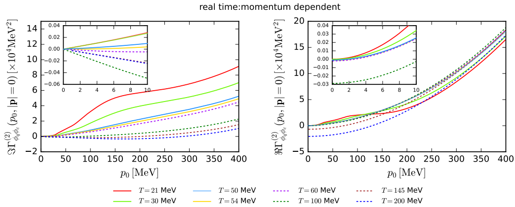
Figure 11: Imaginary (left panel) and real (right panel) parts of the two-point correlation function \Gamma_{\phi_q \phi_c}^{(2)}(p_0, |\mathbf{p}| = 0) as functions of p_0 with several values of temperature. The inlays show the zoomed-in view in the region of small p_0 .
