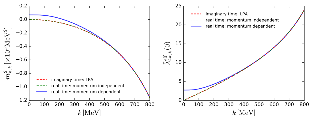
Figure 5: Meson mass square of the effective potential m_{\pi,k}^2 (left panel) in Equation (9) as well as Equation (67) and the effective four-meson coupling \bar{\lambda}_{4\pi,k}^{\text{eff}}(0) with vanishing momenta (right panel) in Equation (66) as functions of the RG scale k in the O(4) scalar theory with temperature T = 145 MeV and initial values of the flow equations at UV cutoff \Lambda = 800 MeV as follows: m_{\pi,k=\Lambda}^2 = -(341.45 \text{ MeV})^2 and \lambda_{4\pi,k=\Lambda} = 24 , where the expectation value of the field \phi_c in Equation (4) is chosen to be vanishing. The red dashed lines denote the results obtained in LPA calculation in the imaginary-time formalism, while the blue solid and green dashed lines stand for those obtained in the real-time formalism, with or without the momentum dependence of the effective four-meson coupling \bar{\lambda}_{4\pi,k}^{\text{eff}} in the self-energy in Equation (64) included, respectively. Note that in order to facilitate the comparison, the contribution from six-point correlations to the flow of four-point vertex in the imaginary-time formalism is neglected.
