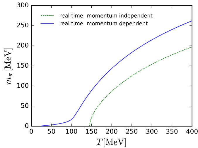
Figure 6: Mass in the infrared limit m_{\pi,k=0} as a function of temperature. The initial conditions for the flows are given by the UV cutoff \Lambda = 800 \text{ MeV} , m_{\pi,k=\Lambda}^2 = -(341.45 \text{ MeV})^2 , and \lambda_{4\pi,k=\Lambda} = 24 . The two different lines denote those obtained in the real-time formalism, with or without the momentum dependence of the effective four-meson coupling \bar{\lambda}_{4\pi,k}^{\text{eff}} in the self-energy in Equation (64) included, respectively.
