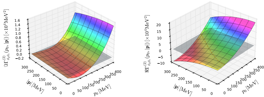
Figure 10: 3D plots of the imaginary (left panel) and real (right panel) parts of the two-point correlation function \Gamma_{\phi_q \phi_c}^{(2)}(p_0, |\mathbf{p}|) as functions of p_0 and |\mathbf{p}| with temperature T = 145 MeV. Here the zero planes, i.e., those with the z -axis z = 0 , are also shown to guide the eyes. The two surfaces intersect with each other at the red dashed line.
