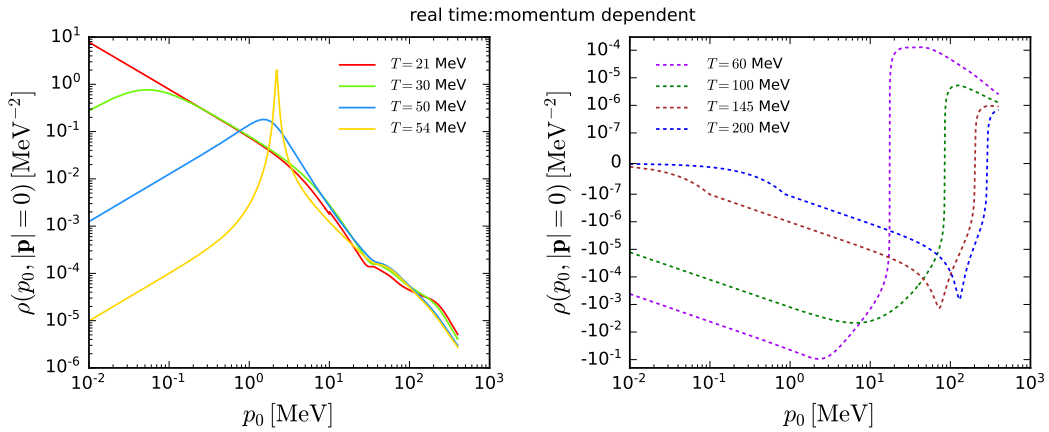
Figure 12: Spectral function \rho(p_0, |\mathbf{p}| = 0) as a function of p_0 with several small (left panel) and large (right panel) values of temperature. In the right panel, a symmetric log scale is applied for the y-axis in order to take into account both positive and negative values of the spectral function, where the log scale is implicitly translated into a linear one upon crossing the zero point.
