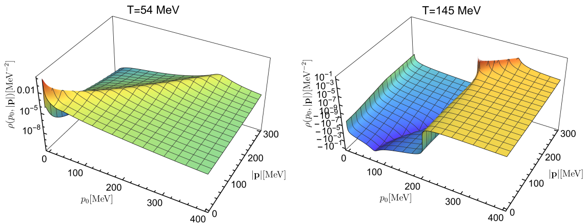
Figure 13: 3D plots of the spectral function as a function of p_0 and |\mathbf{p}| with temperature T = 54 MeV (left panel) and 145 MeV (right panel).
