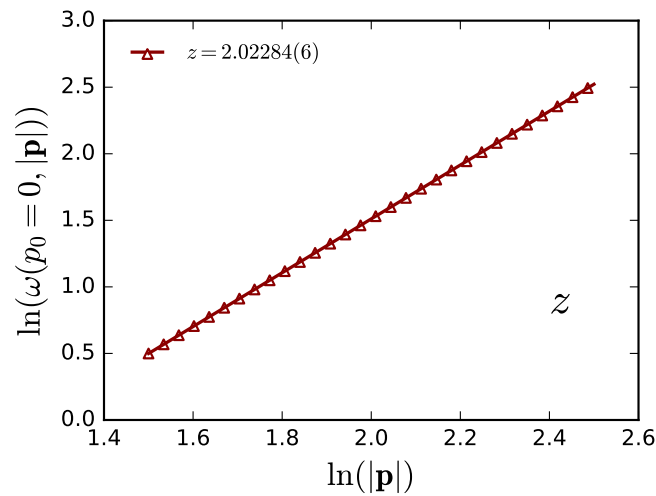
Figure 14: Double logarithm plot of the dissipative characteristic frequency \omega(|\mathbf{p}|) in Equation (86) as a function of the spatial momentum with temperature T = T_c = 20.4 MeV.
