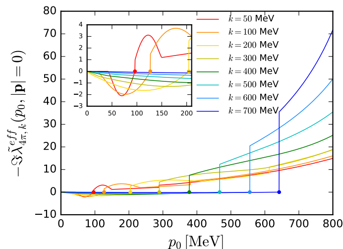
Figure 7: Imaginary part of -\tilde{\lambda}_{4\pi,k}^{\text{eff}}(p_0, |\mathbf{p}|=0) defined in Equation (75) as a function of p_0 with temperature T = 145 MeV, where the spacial momentum is chosen to be vanishing. The mass square m_{\pi,k}^2 in Equation (28) and \lambda_{4\pi,k} in Equation (62) are input from the results of self-consistent computation including the momentum dependence as shown by the solid blue lines in Figure 5. Different lines correspond to difference values of the RG scale k . The inlay shows the zoomed-in view in the region of small p_0 .
