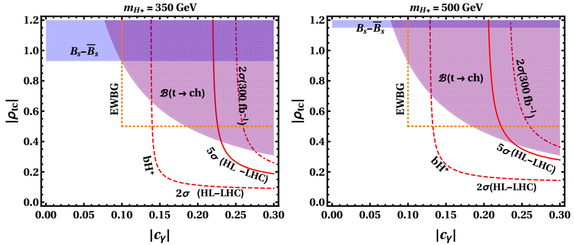
Figure 4: Projected 300 fb -1 exclusion (dot-dashed) and HL-LHC discovery (solid) and exclusion (dashed) contours for the charged Higgs signature pp \rightarrow bH^+ \rightarrow bW^+h , along with EWBG-favored region and the indirect constraints from Fig. 2.
