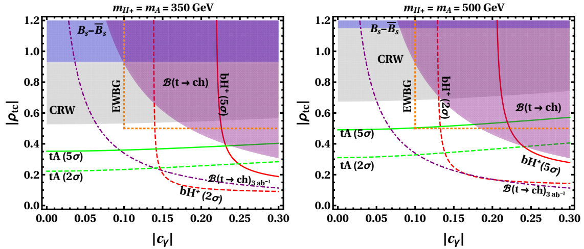
Figure 5: Exclusion regions from neutral Higgs production contributing to the CMS CRW [98] (gray shades), as well as HL-LHC expectations from a dedicated same-sign top search [103] (green). We also show the EWBG region and the indirect constraints from Fig. 2 and the HL-LHC charged Higgs reach from Fig. 4.
