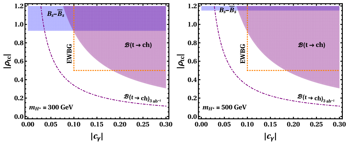
Figure 2: Indirect constraints from B_s - \bar{B}_s mixing (blue), \mathcal{B}(t \rightarrow ch) (purple) in the \rho_{tc} - c_\gamma plane for two H^+ mass values, together with the baryogenesis region (orange).
